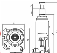
Hydraulic Bottle Jack
