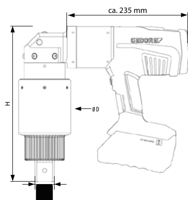
LAW Solution series – angled version
